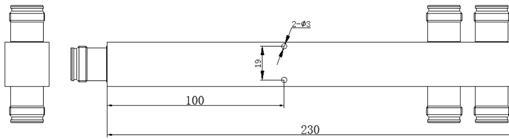
4 Way Splitter
