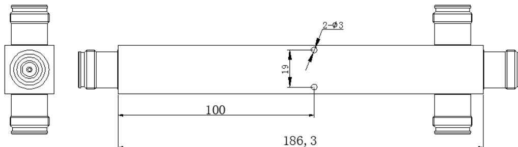
3 Way Splitter
