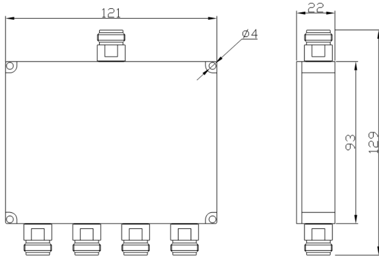
4 Way splitter
