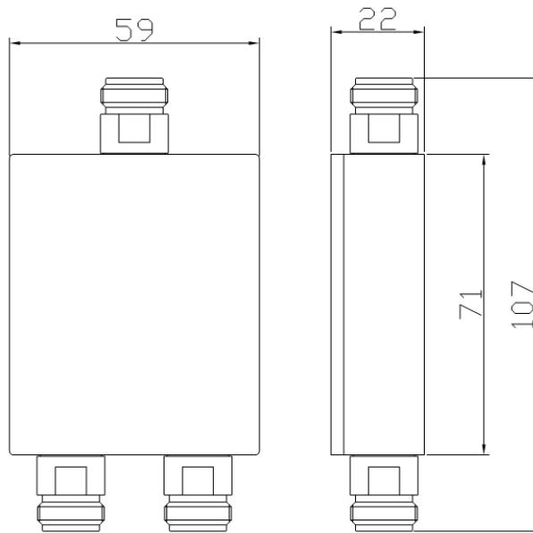
2 Way splitter
