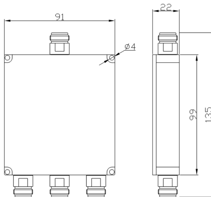
3 Way splitter
